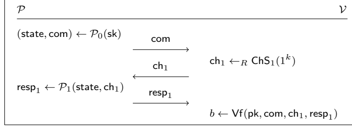
Fig. 1.1: Canonical 3-pass IDS
