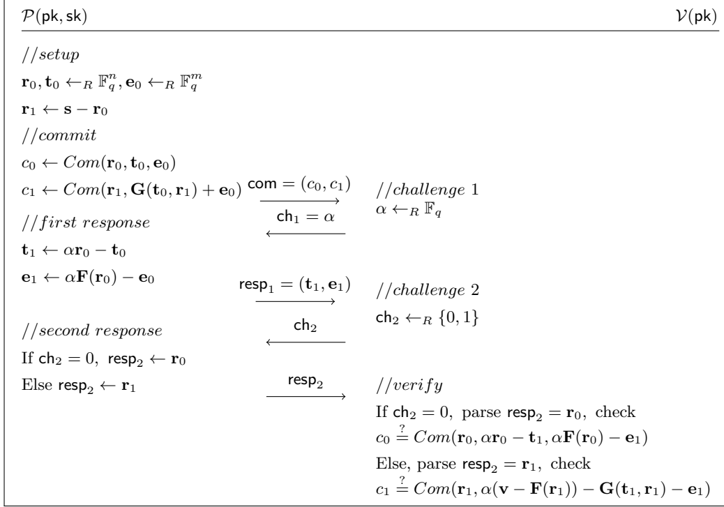
Fig. 3.1: The SSH 5-pass IDS by Sakumoto, Shirai, and Hiwatari [40]
